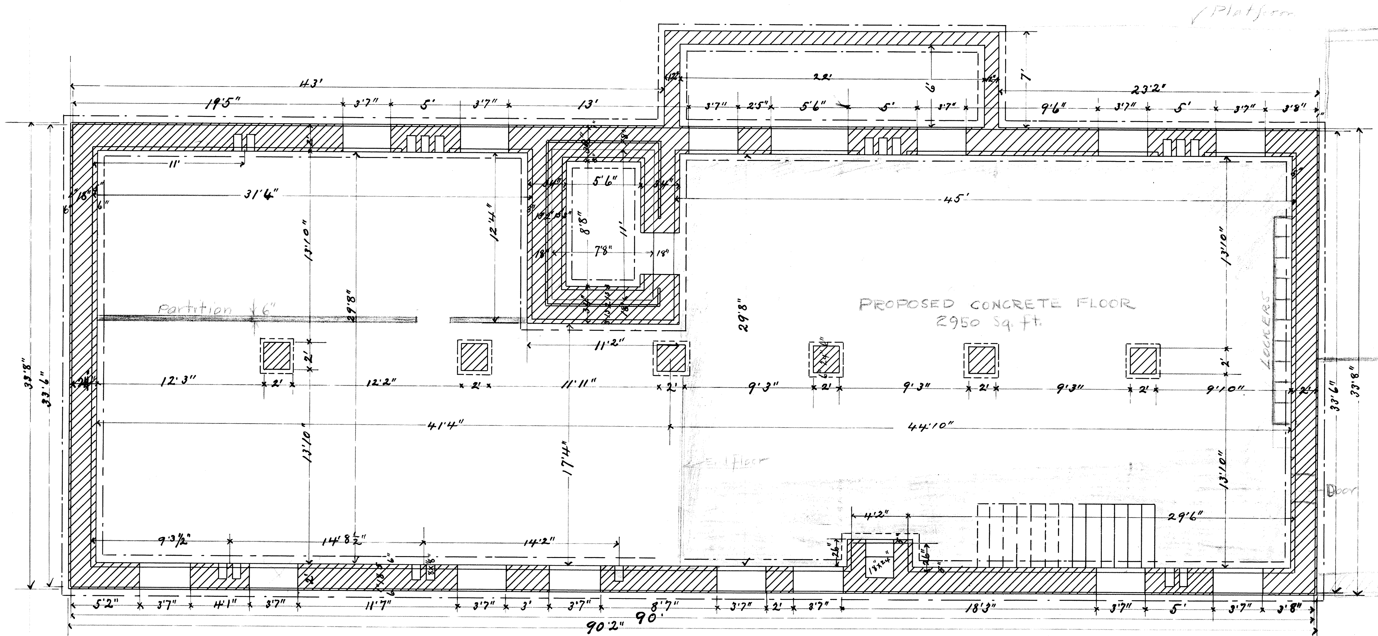
FOUNDATION PLAN AND BASEMENT
